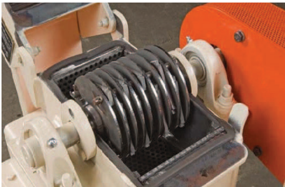
9" rotor diameter features swinging or fixed mounted hammers.
