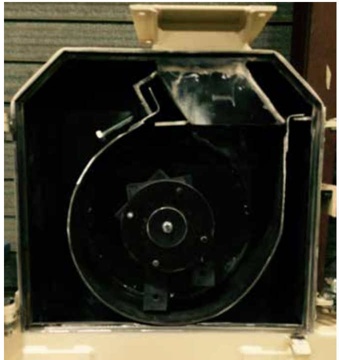
300 degree screen coverage of rotor allows for the highest throughput to horsepower ratio of all hammer mill styles.
